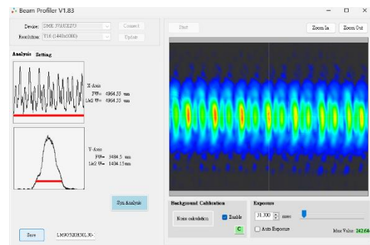
LM9 series Green Line Shape at 1000mm
