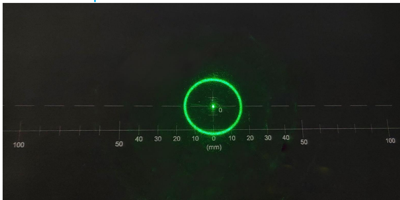
LM9G520H10P39 Beam Shape at 1m
